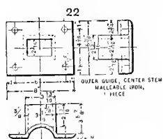
Figs. 1407-1409. Outer Center-stem Guide.
